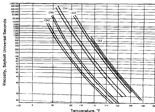
Fig. 4 — Viscosity Ranges of Some Aroclor® Plasticizers
