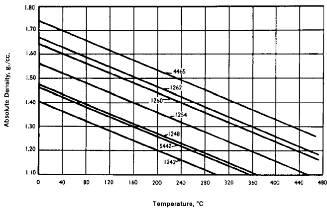
Fig. 2 — Densities of Aroclor® Plasticizers at Various Temperatures
