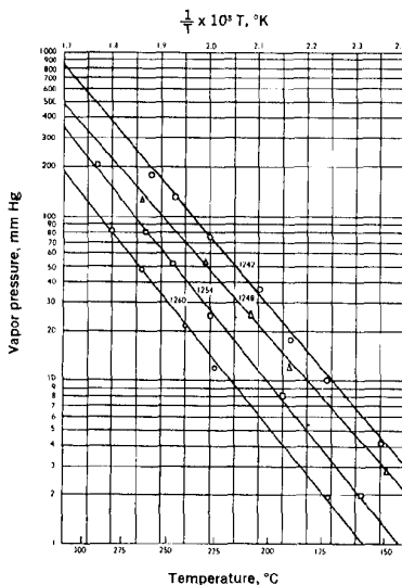
Fig. 3 — Vapor Pressures of Aroclor® Plasticizers
