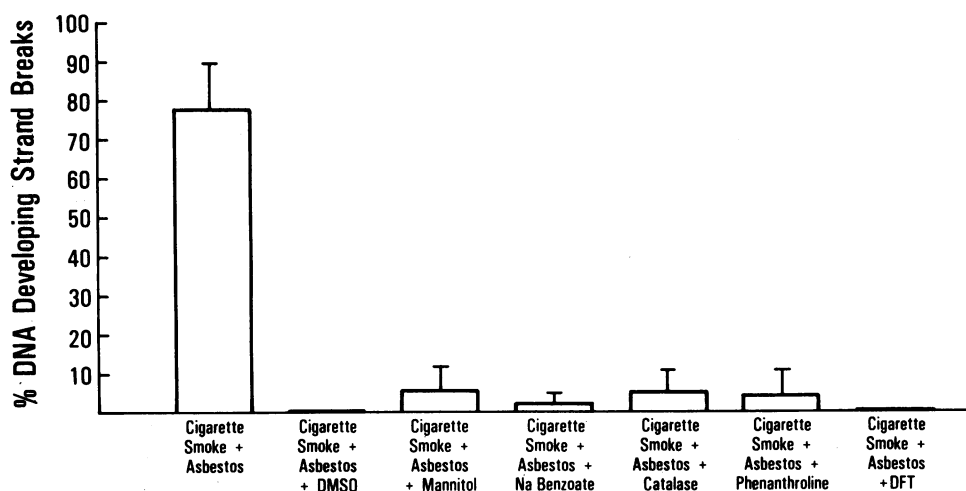
Figure 2. Inhibition of cigarette smoke and asbestos-mediated DNA strand breaks by ^{\circ}\text{OH} scavengers, catalase, or iron chelators. Reaction mixtures and conditions were identical to those in Fig. 1, except for the addition of 100 mM DMSO, 100 mM mannitol, 100 mM Na benzoate, 3.5 \mu\text{g} catalase, 4 mM 1,10-phenanthroline, or 4 mM DFT. Values are means \pm SD. Each value represents four separate experiments performed in triplicate. Values for mixtures containing DMSO, mannitol, Na benzoate, catalase, PHEN, or DFT are all significantly less ( P < 0.05 ) than values for mixtures without these additions.
