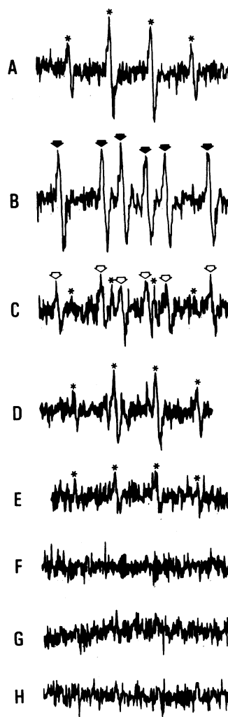
Figure 4. Inhibition of ^{\circ}\text{OH} production by ^{\circ}\text{OH} scavengers, catalase, or iron chelators. Reaction mixtures are identical to those in Fig. 2, except for the addition of 100 mM DMPO. Tracings are EPR spectra of DNA mixtures containing cigarette smoke, asbestos, and the following components: (A) no additional components, (B) ethanol (6.5 M), (C) DMSO, (D) mannitol, (E) Na benzoate, (F) catalase, (G) PHEN, (H) DFT. (*, DMPO-OH signal; closed arrows, DMPO-alpha-hydroxyethyl radical signal; and open arrows, DMPO- \text{CH}_3 signal.)
