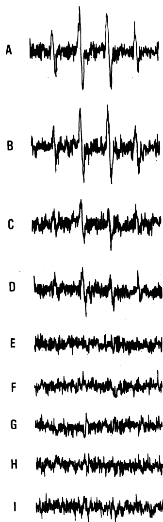
Figure 3. ^{\circ}\text{OH} production in various DNA mixtures. Reaction mixtures are identical to those in Fig. 1, except for the addition of 100 mM DMPO. Tracings are EPR spectra obtained immediately after the addition of all reaction components. (A) DNA + cigarette smoke + asbestos, (B) DNA + cigarette smoke + \text{FeSO}_4 , (C) DNA + \text{H}_2\text{O}_2 + asbestos, (D) DNA + \text{H}_2\text{O}_2 + \text{FeSO}_4 , (E) DNA alone, (F) cigarette smoke alone, (G) asbestos alone, (H) \text{FeSO}_4 alone, (I) \text{H}_2\text{O}_2 alone.
