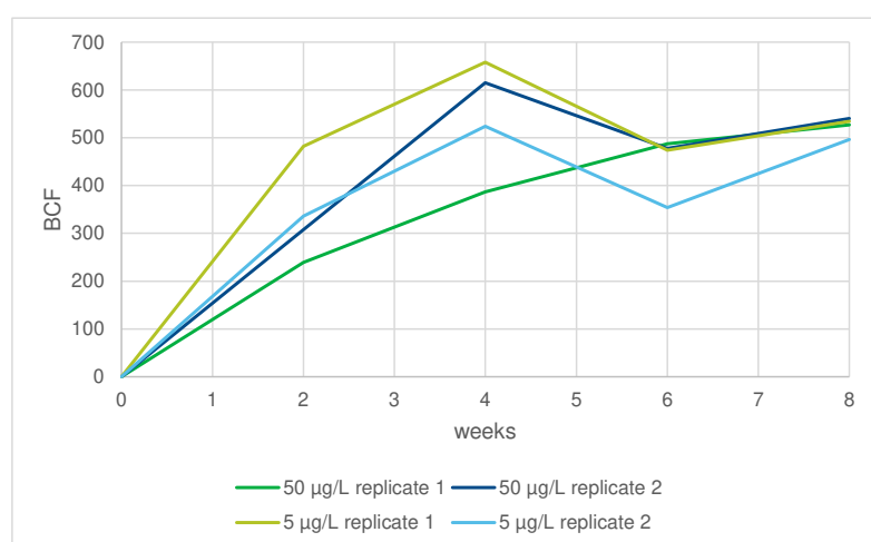
Figure 6.2 BCF over time (weeks) for each replicate
