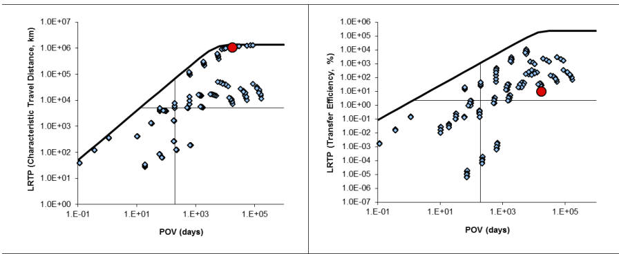
Figure 6.1 Long range transport potential of 1H-perfluorohexane
