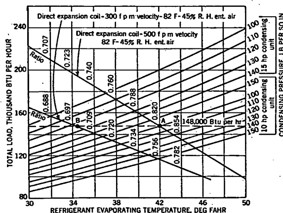
FIG. 11. COMPRESSOR AND COIL PERFORMANCE
