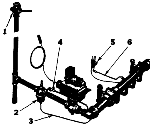
FIG. 18—Control Connections
