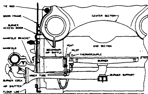
FIG. 7—Burner No. 2 and Pilot Installation-Manual Ignition
