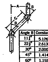
FIG. 19. CONSTANTS FOR DETERMINING LENGTH OFFSET PIPE
