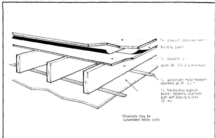
Figure 1. One-hour assembly – resilient channel ceiling system.
