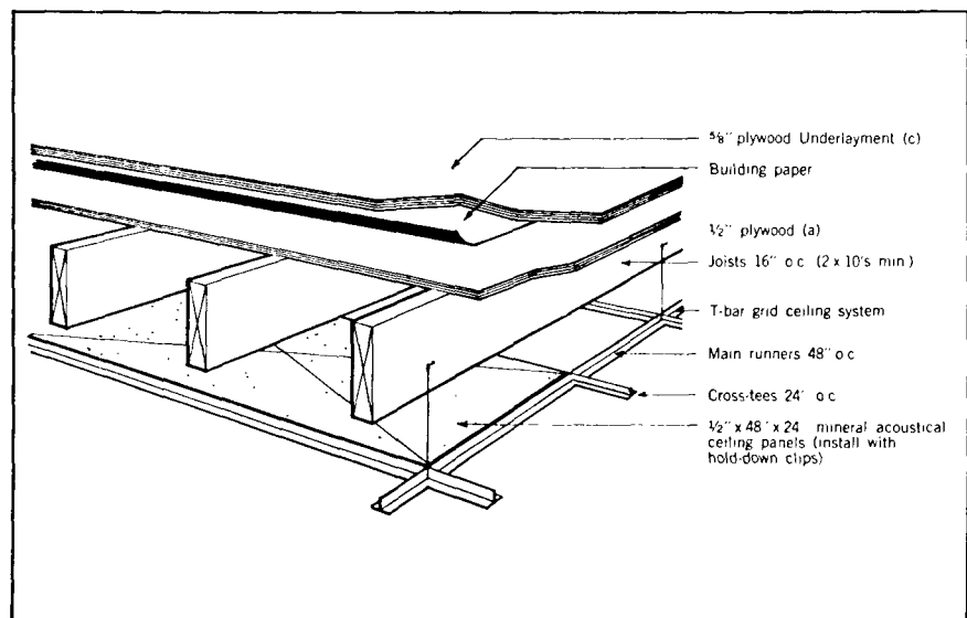
Figure 2. One-hour assembly – T-bar grid ceiling system.
