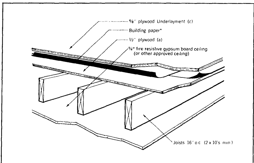
Figure 3. One-hour assembly – ceiling attached directly to joists.
