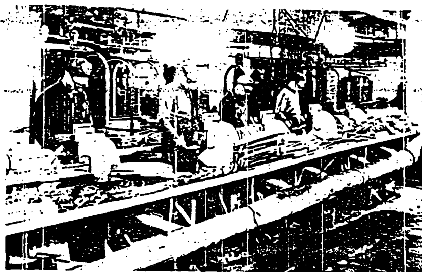
Figure 3 Each of these grinding wheels is partially enclosed by an exhaust hood. Efficient local exhaust is achieved by drawing the dust into the hoods, through branch ducts, and into a central duct which leads to the collection point. (Courtesy American Foundrymen's Society.)
