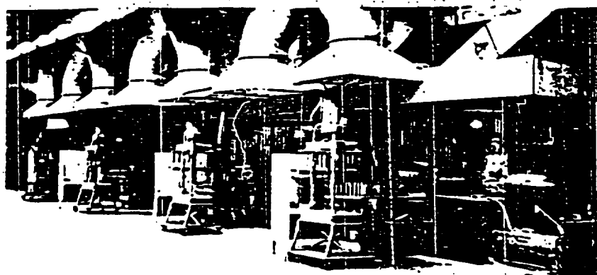
Figure 7. In this foundry, local exhaust hoods are installed over each station having a shell-molding machine and glue press. Adequate make-up air is supplied from ventilating duct situated between molding machines and presses. (Courtesy American Foundrymen's Society)
