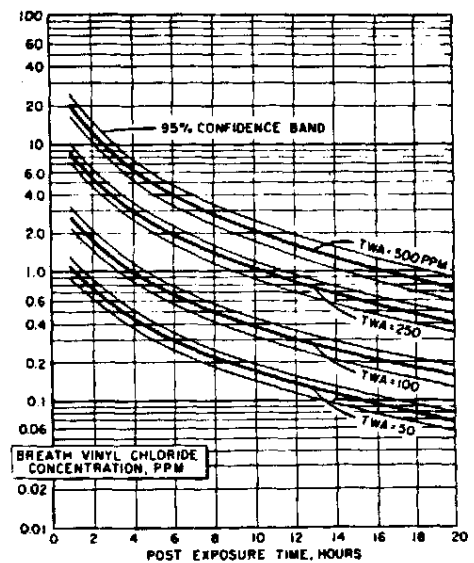
FIGURE 5. Breath decay curves based on experimental human exposures to 50, 250, and 500 ppm of VCl (7.5-hour TWA).
