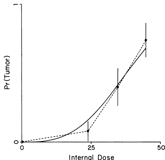
FIGURE 4. Plot of probability of all squamous cell carcinomas versus internal dose for B6C3F 1 male mice with superimposed multistage model fitted curve (solid line). Dashed lines connect the observed quantal responses at each dose value. The quantal response data points along with 95% confidence limits are presented as solid circles with vertical lines.
