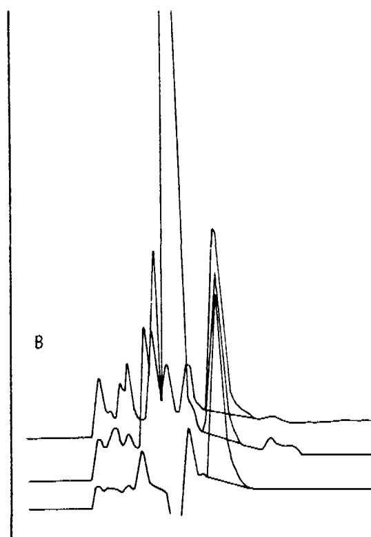
Fig. 2. Mass fragmentogram of the O-methyl ester of N -acetyl- S -(2-hydroxyethyl)cysteine from the urine of chloroacetaldehyde-treated rats (the gains from m/e 144, m/e 162 and m/e 203 are in the ratio 1 : 10 : 10). A represents the injection point for a methanolic solution of the standard sample and B that for the 3 N acetic acid fraction (for details, see Materials and Methods, derived from urinary material). The latter shows all 3 ions with identical relative intensities and retention time as the standard.
