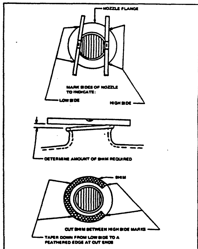
Figure 21. Shimming the Drive Nozzle Gasket
