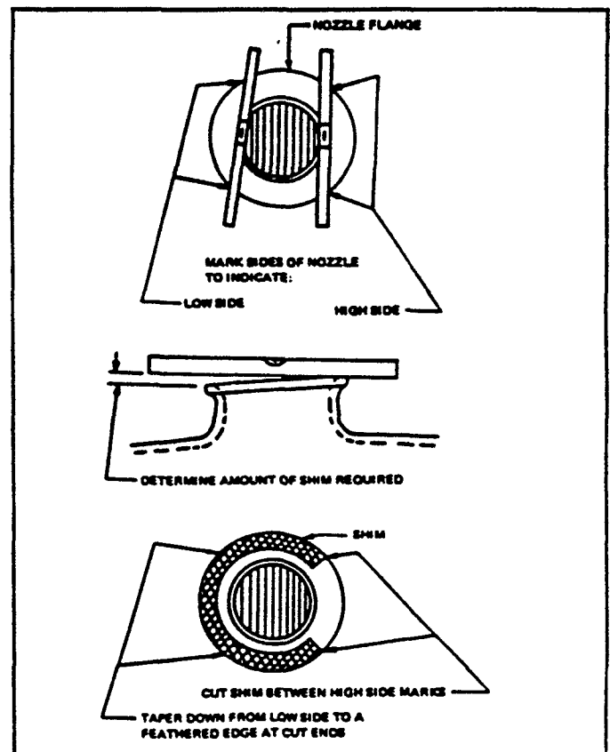
Figure 16. Shimming the Drive Nozzle Gasket
