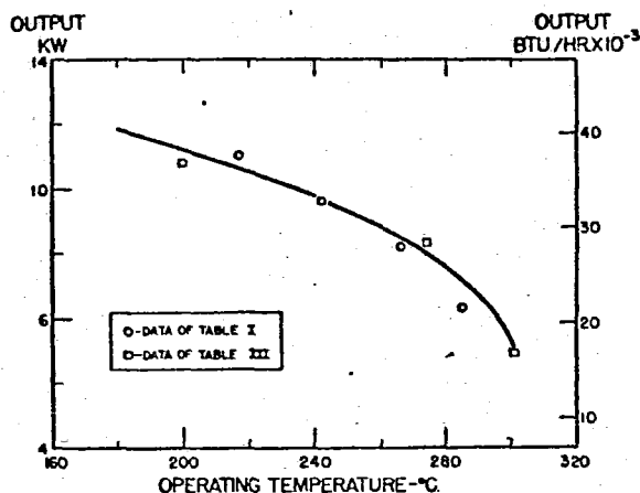
Figure 3. Temperature-Capacity Curve for Portable Aroclor Heater
