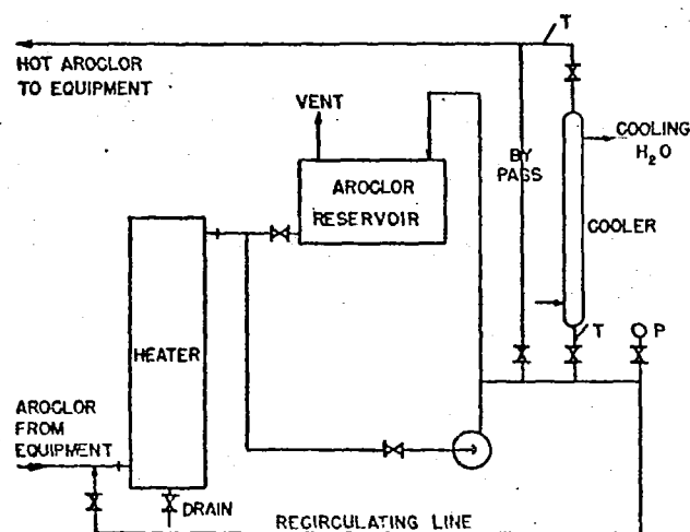
Figure 2. Flow Diagram for Aroclor Heater
