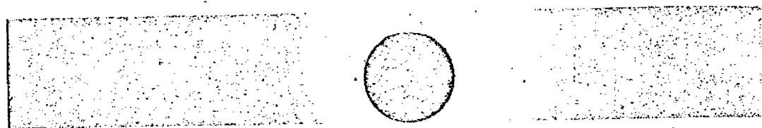
FIG. 6. X-ray diffraction film of lung residue of E. R. * The lines listed when compared to the known pattern for asbestos give positive proof that the lung residue is essentially asbestos.
