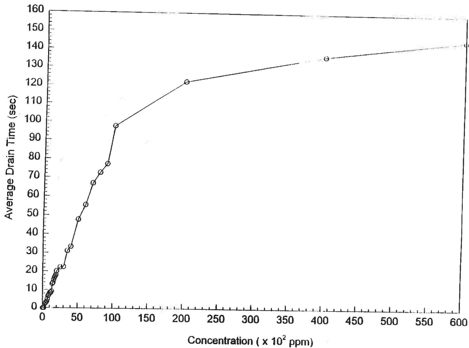
Fig. 2 - Average Drain Time vs. Concentration for AFFF (6%) Solutions
