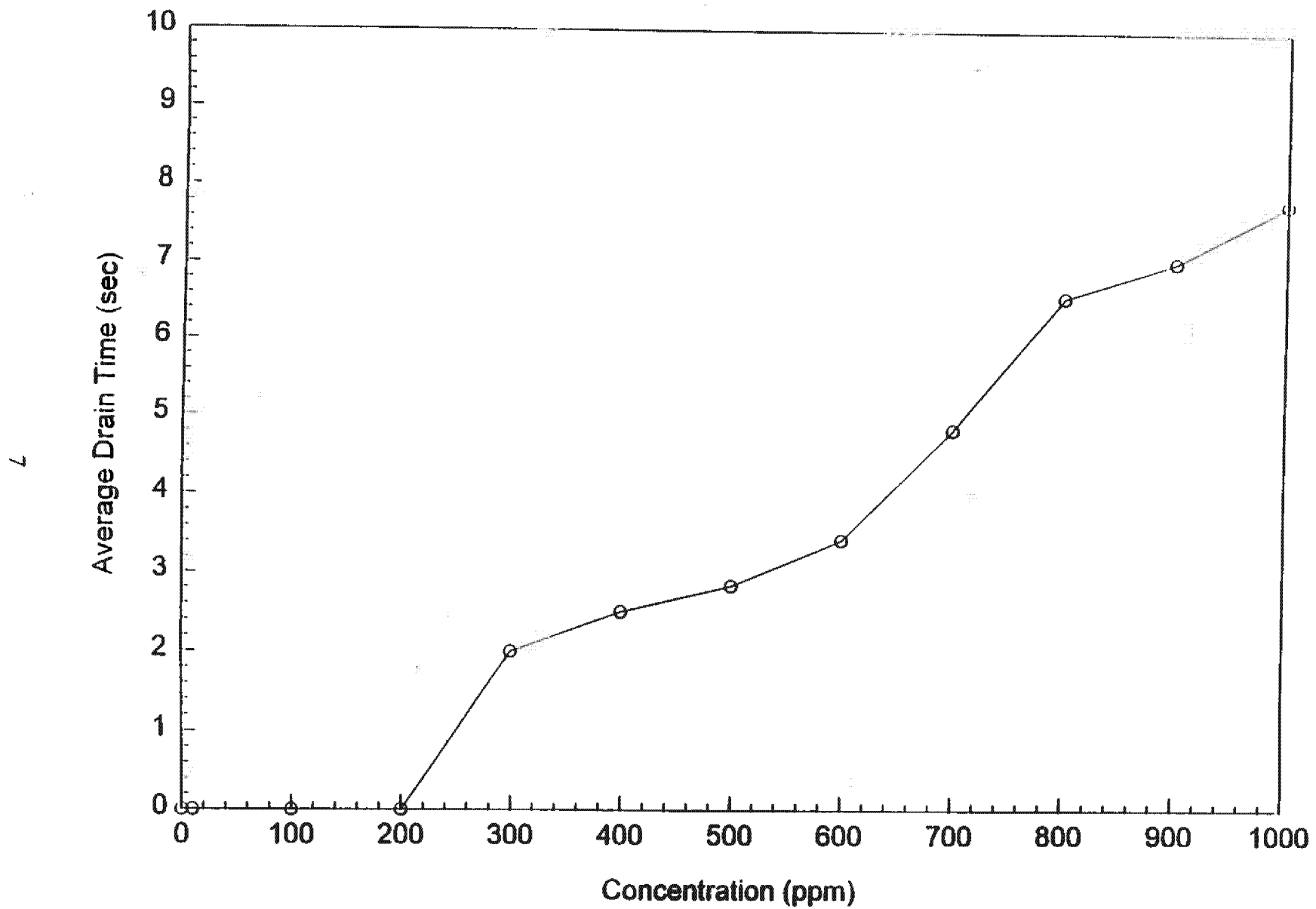
Fig. 1 - Average Drain Time vs. Concentration for AFF (6%) Solutions
