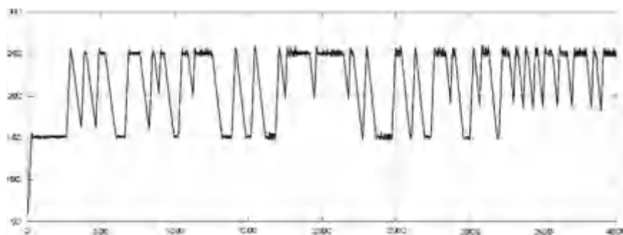
Fig. 2.5 Random step output from the system
