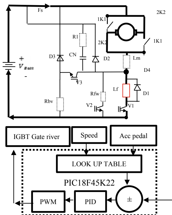
Fig. 20.1 Current paths in reverse mode
