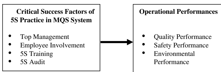
Fig. 29.1 Initial framework
