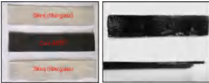
Fig. 1.3 Layers of the MRE composite on the left and MRE sandwich structural plate after attached together on the right
