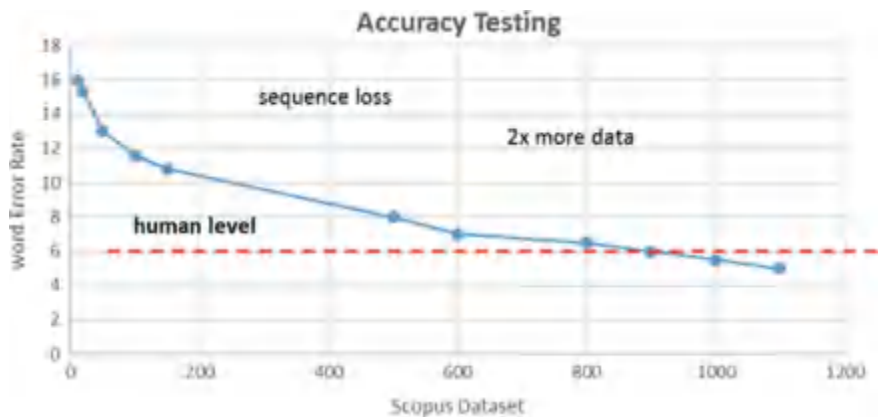
Fig. 6.10 Accuracy testing on different dataset threshold
