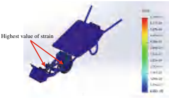
Fig. 30.12 Strain results of wheelbarrow loader bucket
