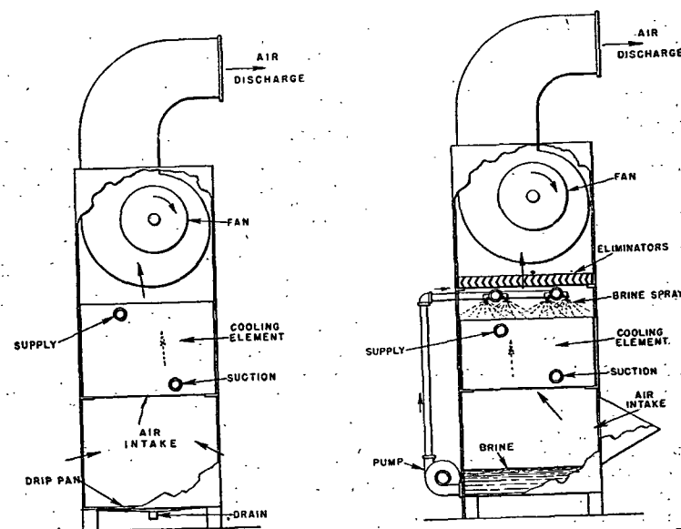
FIG. 9. SURFACE TYPE COOLING UNIT. FIG. 10. BRINE SPRAY TYPE COOLING UNIT.
