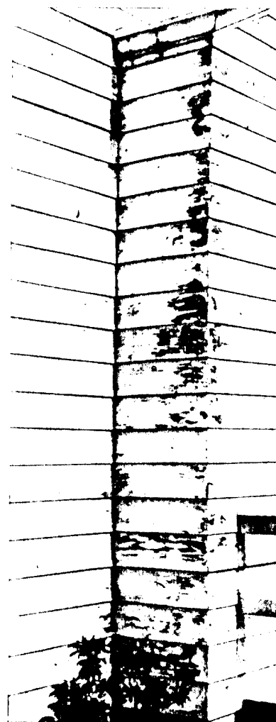
FIGURE 18.—Serious peeling. Peeling is particularly noticeable at corners, where water behind certain parts of siding, probably in winter. At ground level the building is p...
