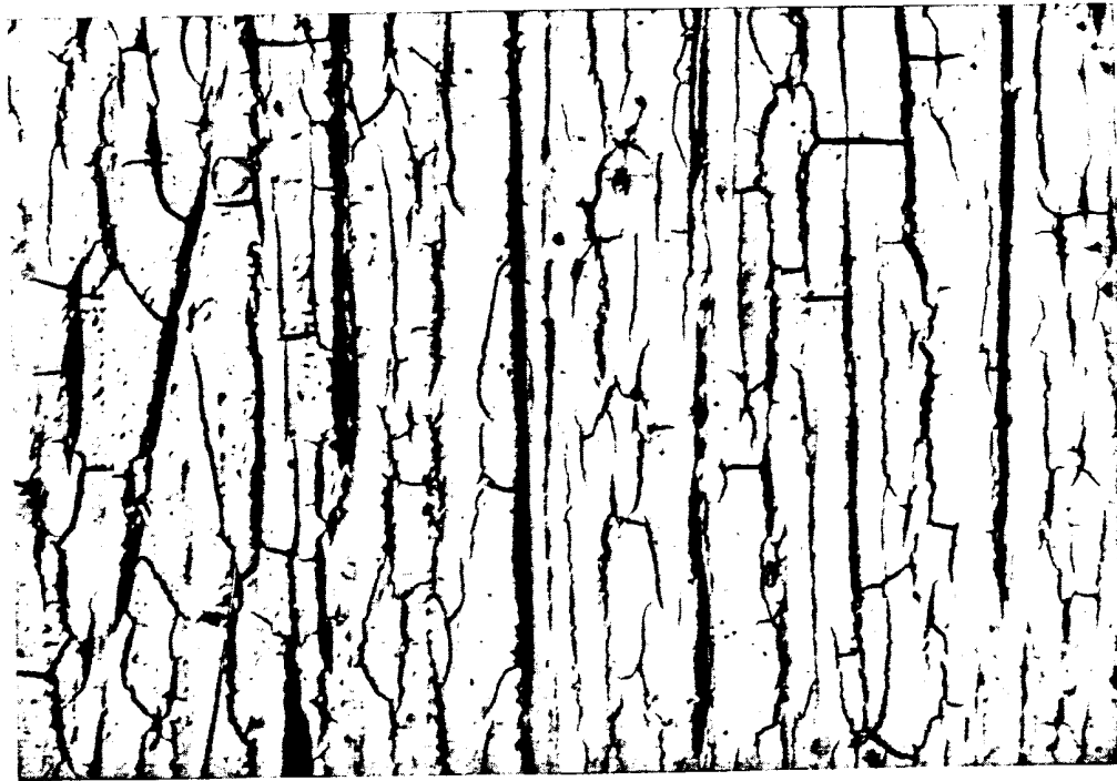
FIGURE 31.—Typical alligatoring of finish coat of white paint (hard type) applied over dark-red paint (soft type).
