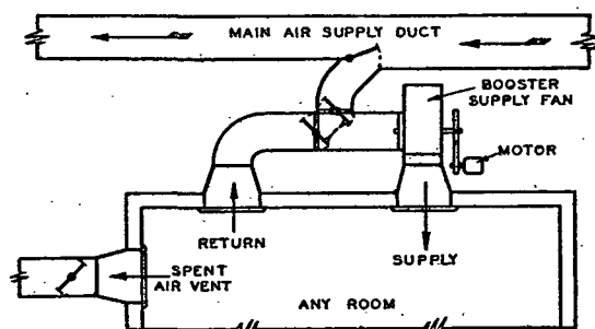
FIG. 3. ARRANGEMENT FOR INDIVIDUAL ROOM TEMPERATURE CONTROL WITH CENTRAL AIR SUPPLY SYSTEM
