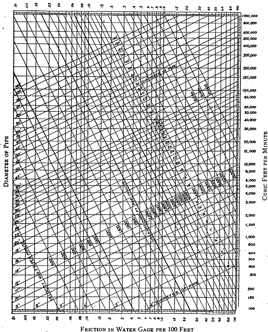
FIG. 77. FRICTION CHART
