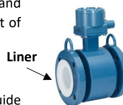
Figure 3. Liner Example.
