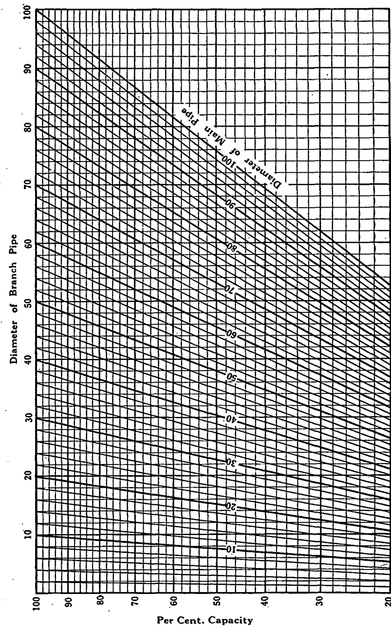
FIG. 3. MAIN AND BRANCH PIPES FOR EQUAL FRICTION PER FOOT OF LENGTH
