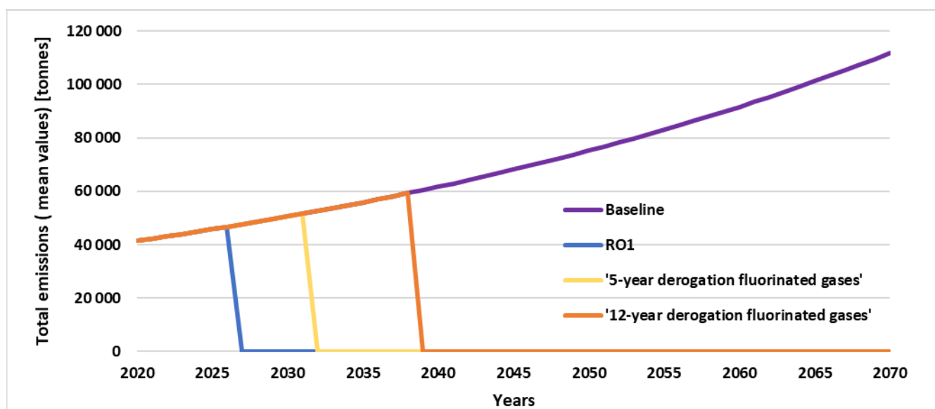
Figure E.13. Time path of mean emissions under the baseline, R01, and maximum additional emission scenario (fluorinated gases sector, in tonnes).
