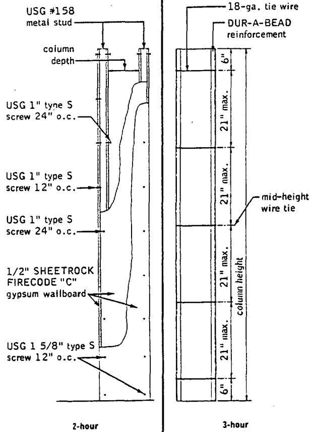
Column elevations
