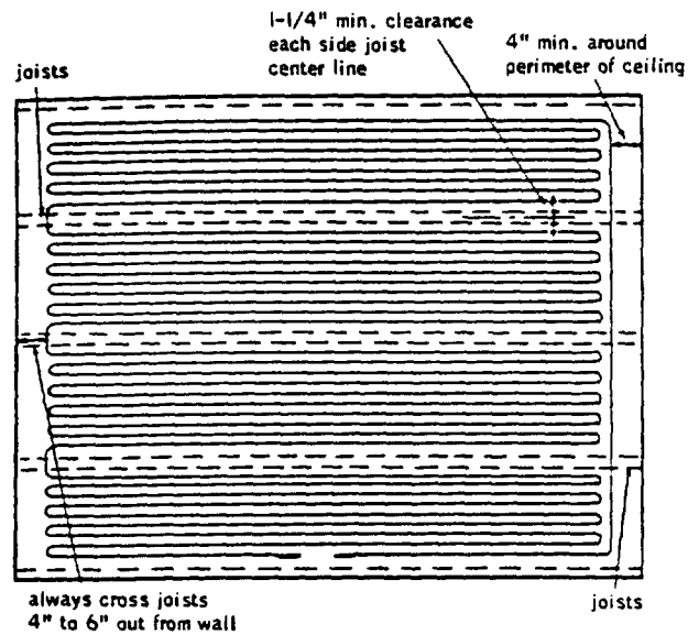
Typical layout—electrical radiant heated ceiling
