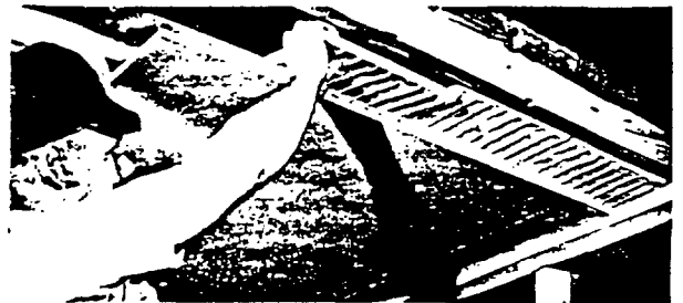
B. Apply wallboard horizontally with long edges at right angles to joists. Place backing blocks along full length of edge and ends of board. Floating of end joints makes it easier to form a good joint over a twisted stud or joist.
