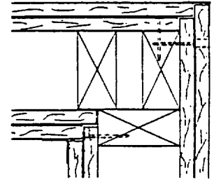
Corner detail
