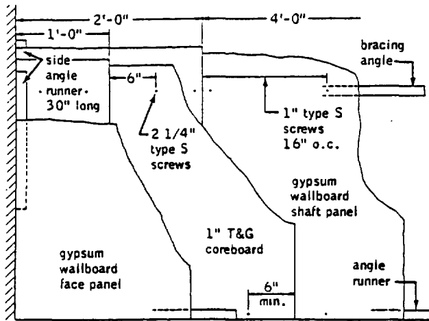
Wall elevation
