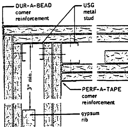
Partition corner
