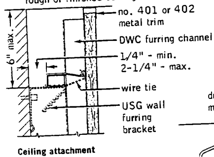
Ceiling attachment
