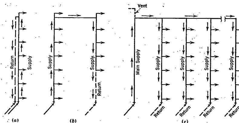
FIG. 11. METHODS OF ARRANGING HOT WATER CIRCULATION LINES
