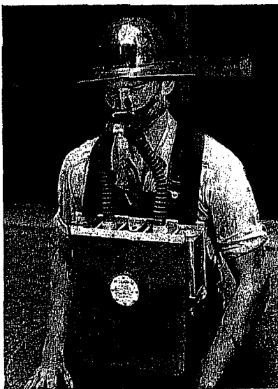
Courtesy, Mine Safety Appliances Co. Figure 1. Self-contained oxygen breathing apparatus provides respiratory protection for one hour in any atmosphere. (See paragraph 6.)
