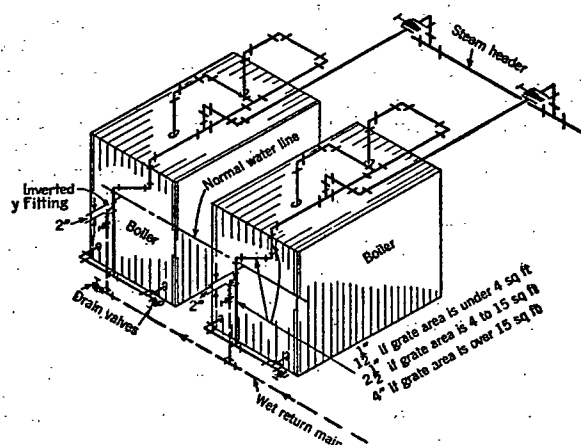
FIG. 20. THE HARTFORD RETURN CONNECTION
