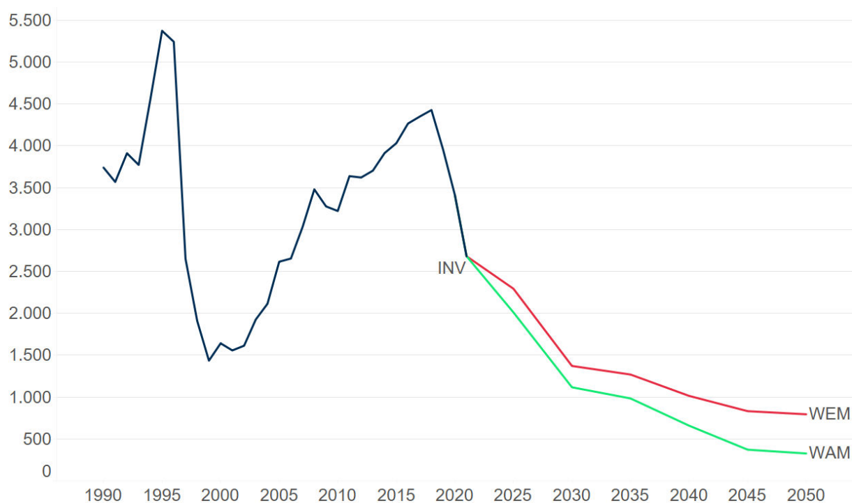
Figure 2-2. Evolution of the F-gas emissions in Belgium (in kt CO 2 -eq).
