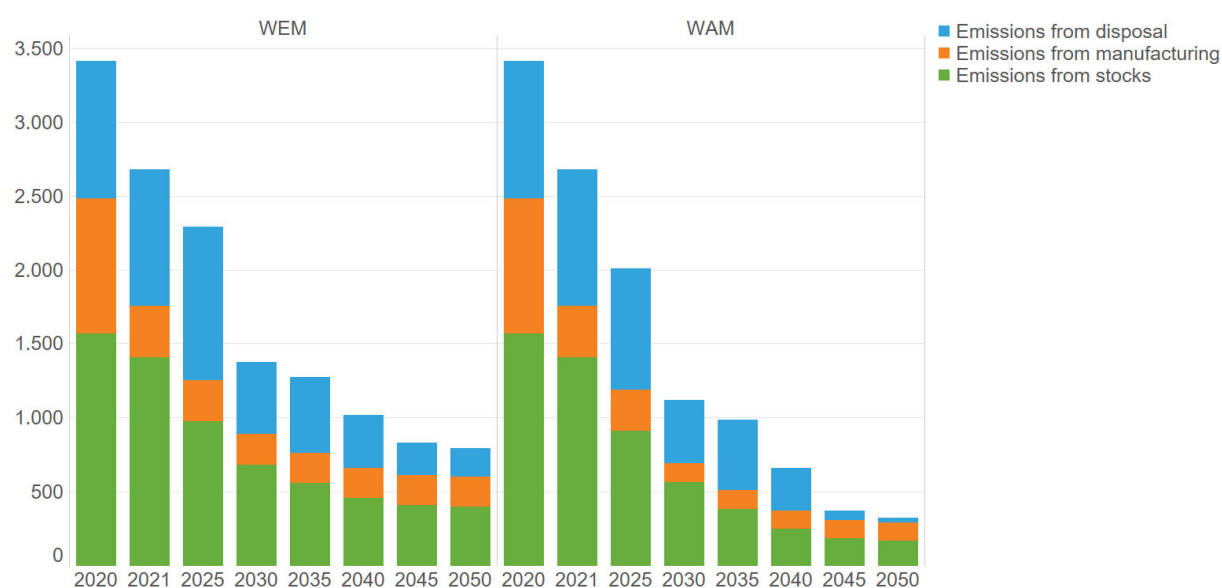
Figure 2-7. Evolution of CRF F-gas emissions from manufacturing, stock and disposal in Belgium (in kt CO 2 -eq).
