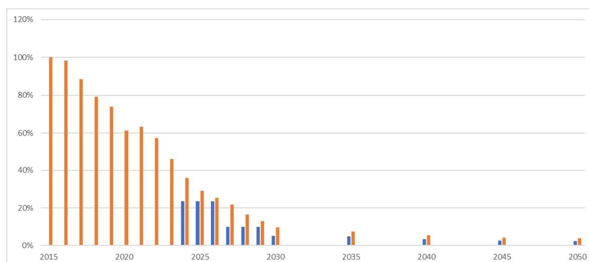
Figure 2-9. Comparison of the phase-down (blue) and the consumption in the WAM scenario (orange) (% consumption in CO 2 -eq).
