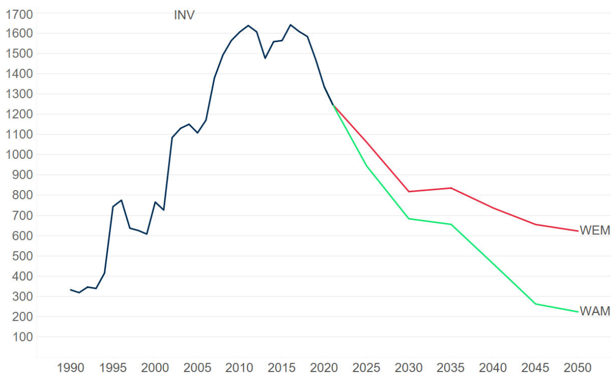
Figure 2-1. Evolution of the CRF F-gas emissions in Belgium (in t).
