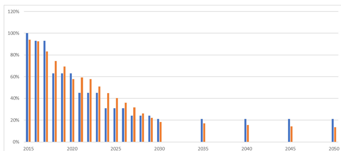
Figure 2-8. Comparison of the phase-down (blue) and the consumption in the WEM scenario (orange) (% consumption in CO 2 -eq).
