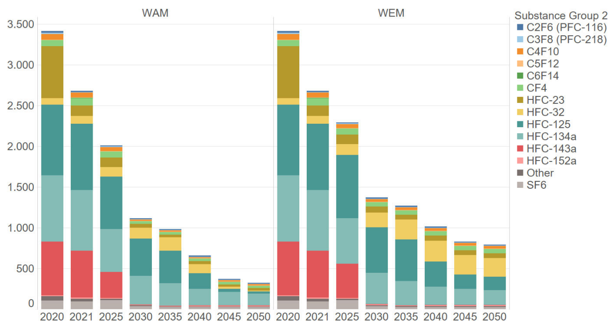
Figure 2-4. Evolution of the CRF F-gas emissions of the most important substances in Belgium (in kt CO 2 -eq).
