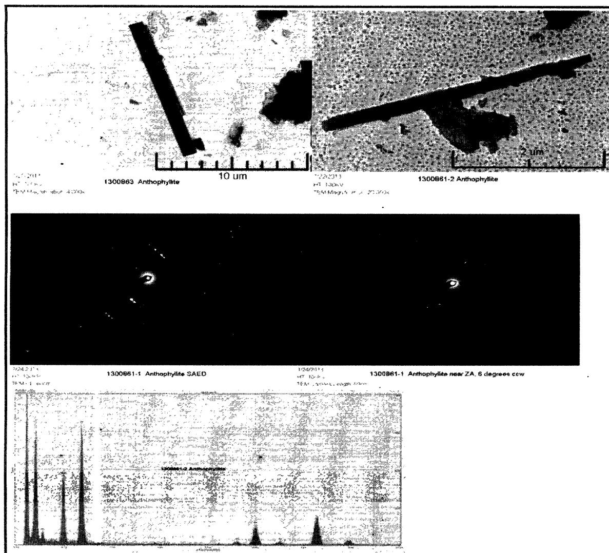
Figure 7 Anthophyllite asbestos from TEM analysis of releasability air testing of product (images, EDS, and SAED).
