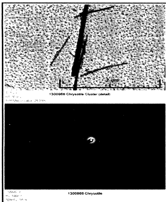
Figure 8 Chrysotile asbestos from TEM analysis of releasability air testing of product (Image and SAED).
