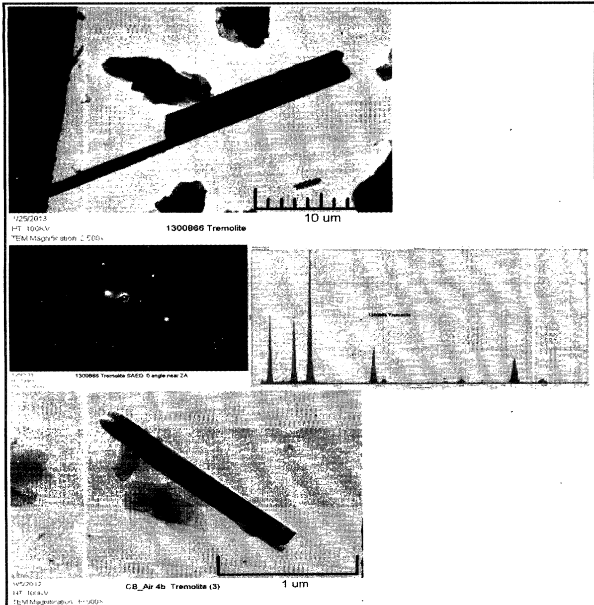
Figure 6 Tremolite asbestos from TEM analysis of releasability air testing of product (images, EDS, and SAED).
