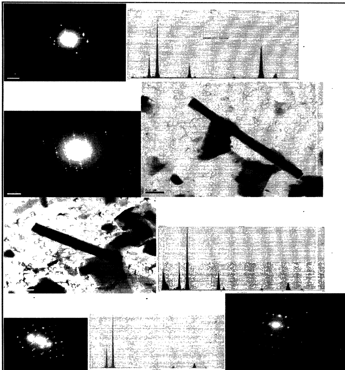
Figure 12 Tremolite and anthophyllite asbestos from re-analyses of 'Lab D' preparations (images, EDS, and SAED).
