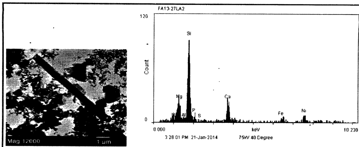
Figure 10 This asbestos fiber is a representative sample removed from the lung tissue of the patient exposed to cosmetic talcum powder. Tremolite asbestos fiber with its corresponding EDS spectra.
