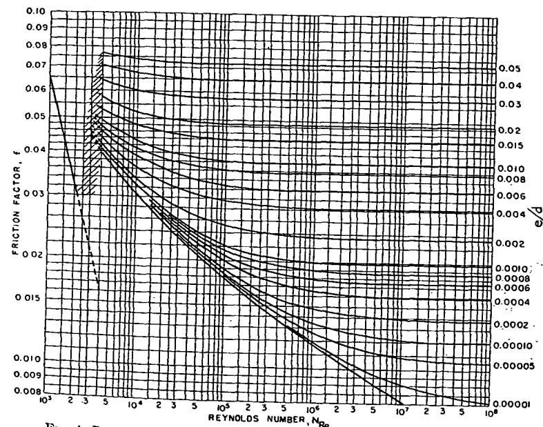
FIG. 4. RELATION BETWEEN FRICTION FACTOR AND REYNOLDS NUMBER NOTE: The straight line at left shows values of Friction Factor for laminar flow. Reprinted by permission from ASME Transactions.
