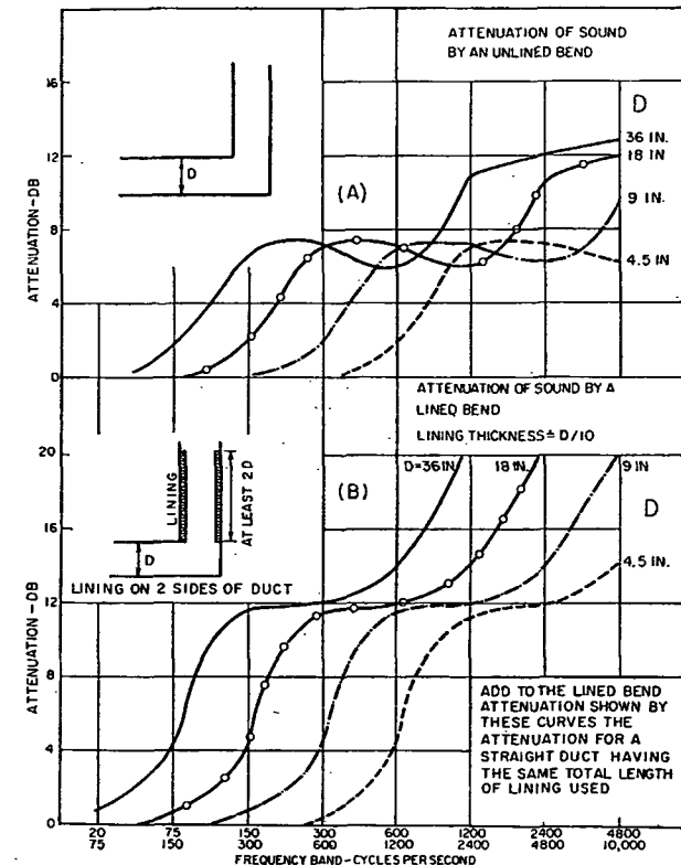
FIG. 8. ATTENUATION IN DECIBELS PROVIDED BY (A) UNLINED BEND, AND (B) LINED BEND IN A DUCT WITH THE LATERAL DIMENSION D
