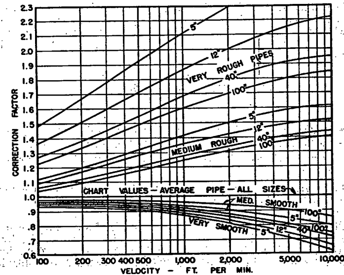
FIG. 3. CORRECTION FACTORS FOR PIPE ROUGHNESS
