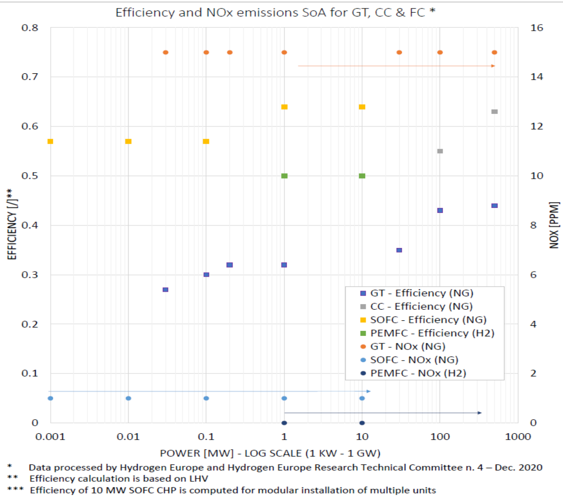
Figure 1 State of the Art net efficiency 126 and NO x emissions for fuel cells and Gas Turbines
