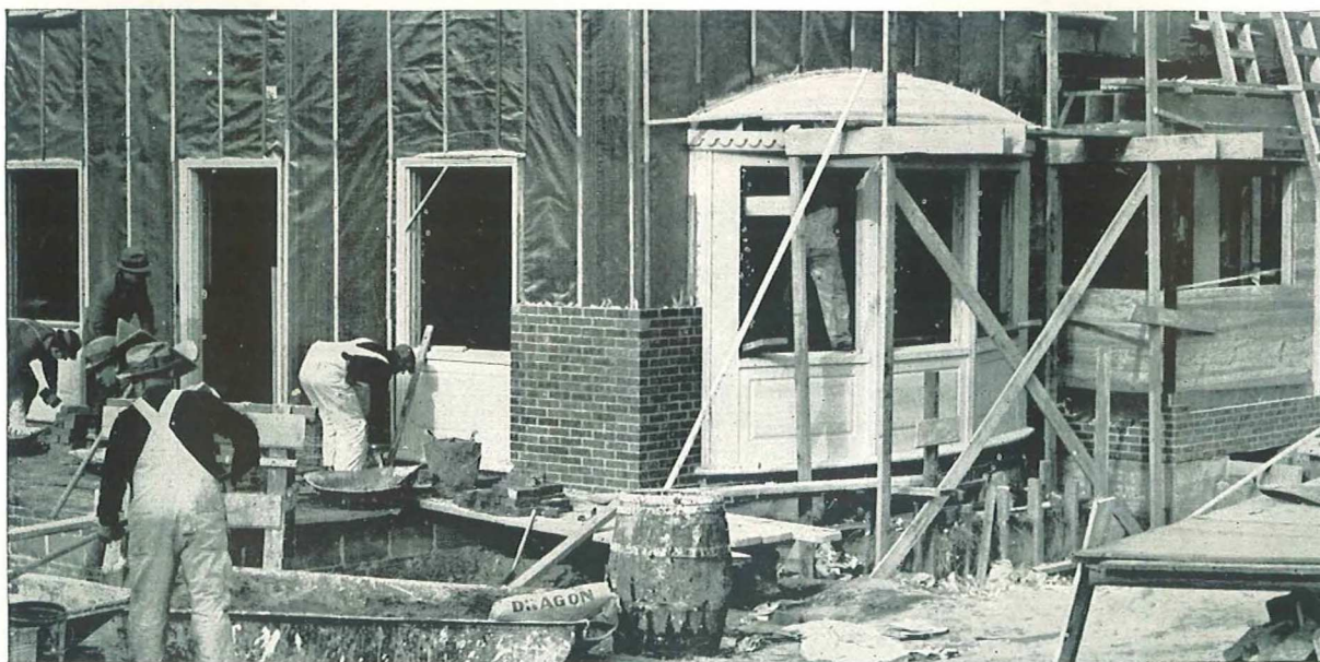
"Electro-Sheet" plain or bonded to building paper will keep air and moisture from penetrating the walls.
