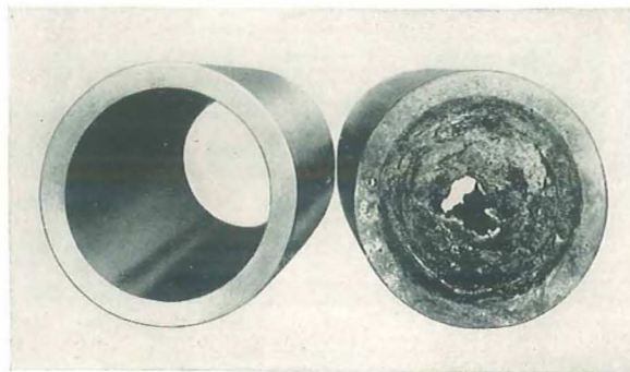
This photograph shows brass pipe (left) and rustable pipe (right) after identical service. This is a graphic illustration of the extent to which rust may interfere with service even though leaks have not developed.
