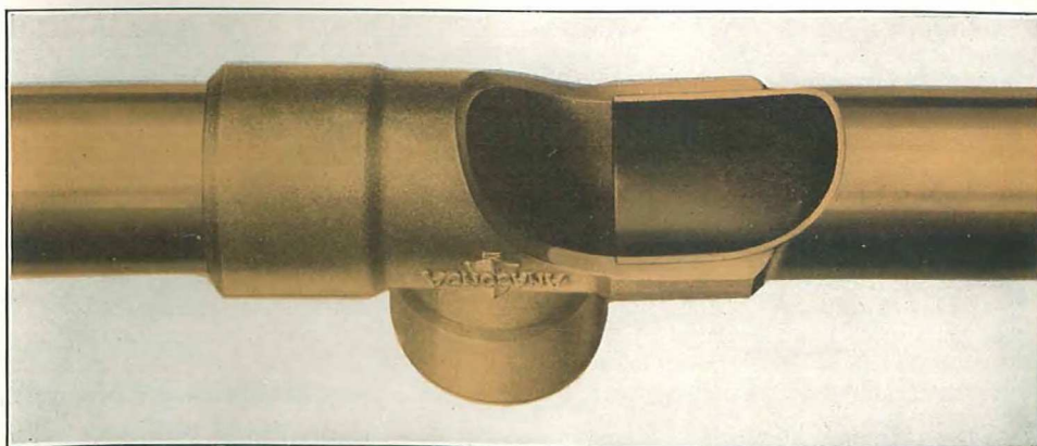
Cut-away section showing completed joint of tube and solder fitting. Note the generous depth of the cup and the accurate fit at the end of the tube. This practically eliminates resistance to the flow of water.
