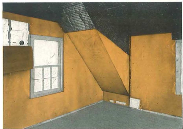
Copper Vapor Seal has been fastened to inside of studs over insulating material. As this room will be plastered, metal lath is shown partially applied (at top) over the copper.
