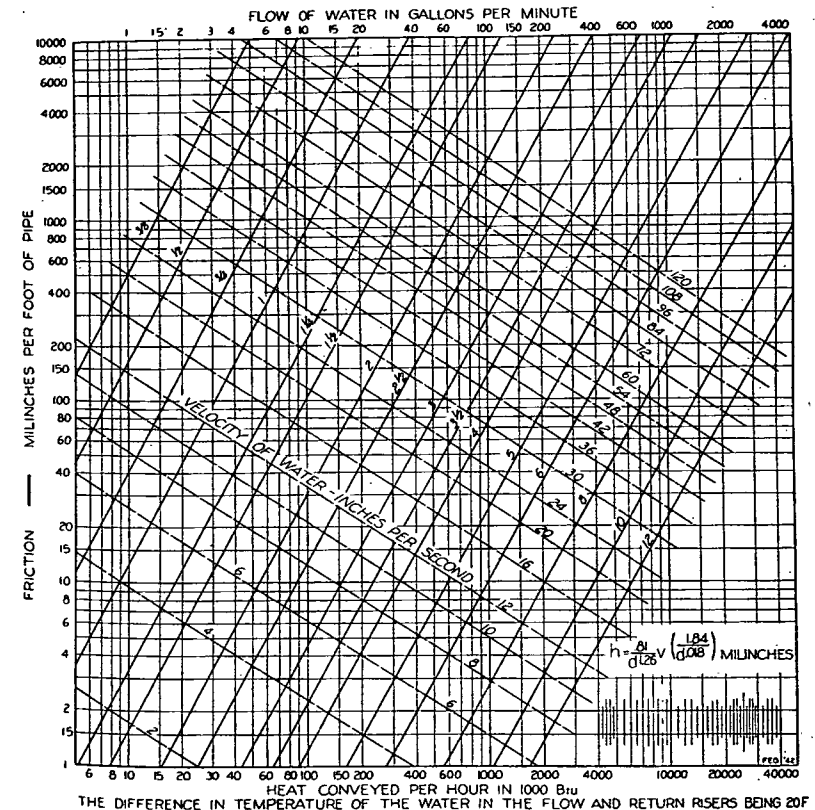
FIG. 2. FRICTION IN BLACK IRON PIPES
