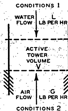
FIG. 10. OPERATIONS IN A TYPICAL WATER COOLING TOWER
