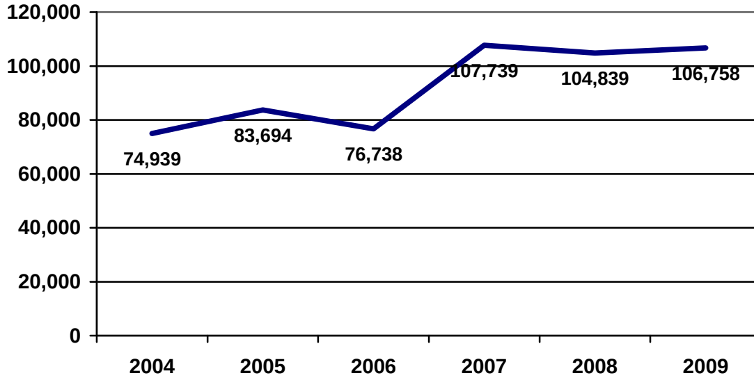
Figure 1-3: Routine Investigations
