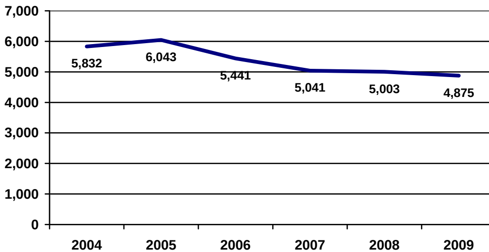
Figure 1-4: Complaints Investigated
