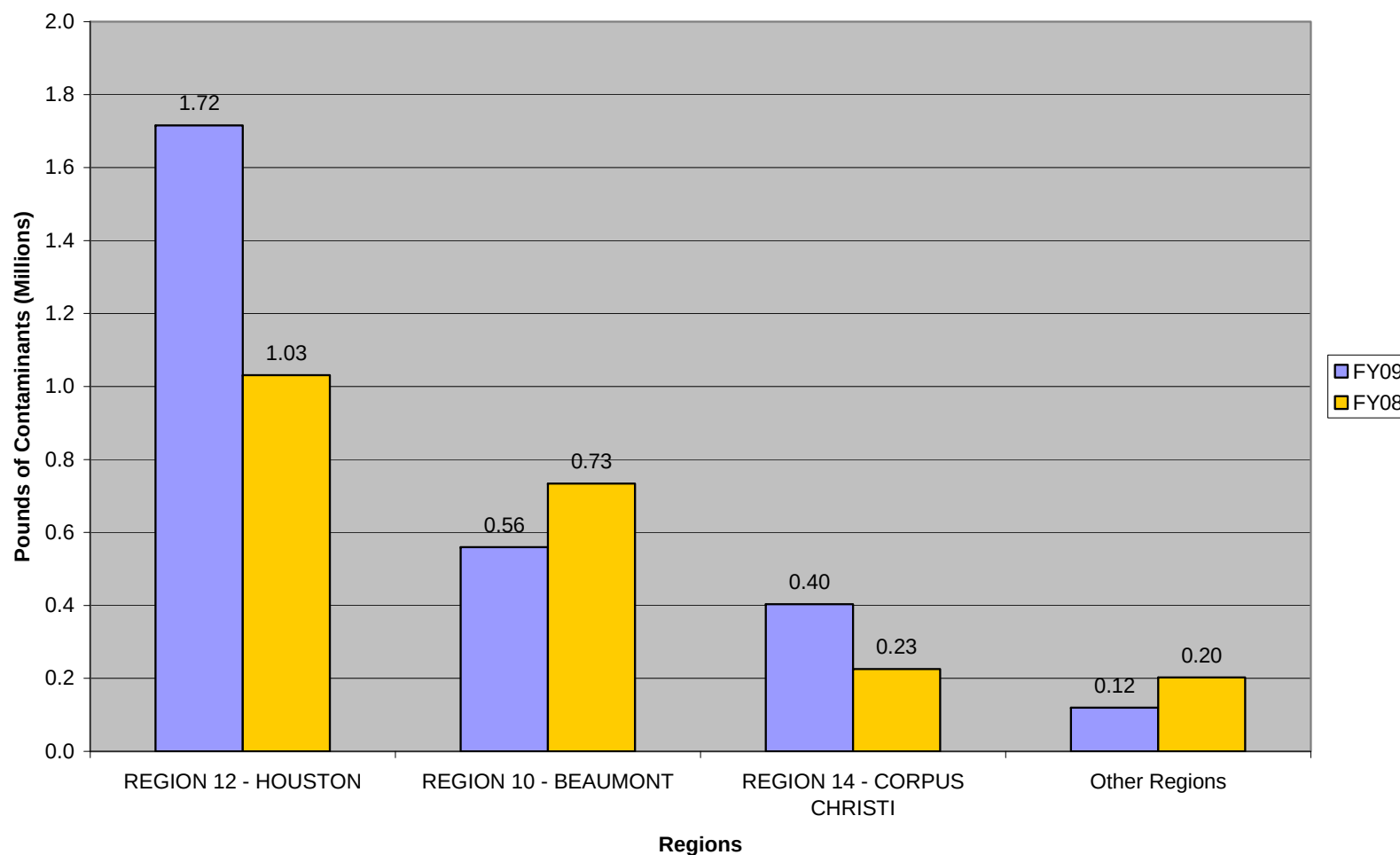
Figure 5-7 Highly-Reactive VOCs
