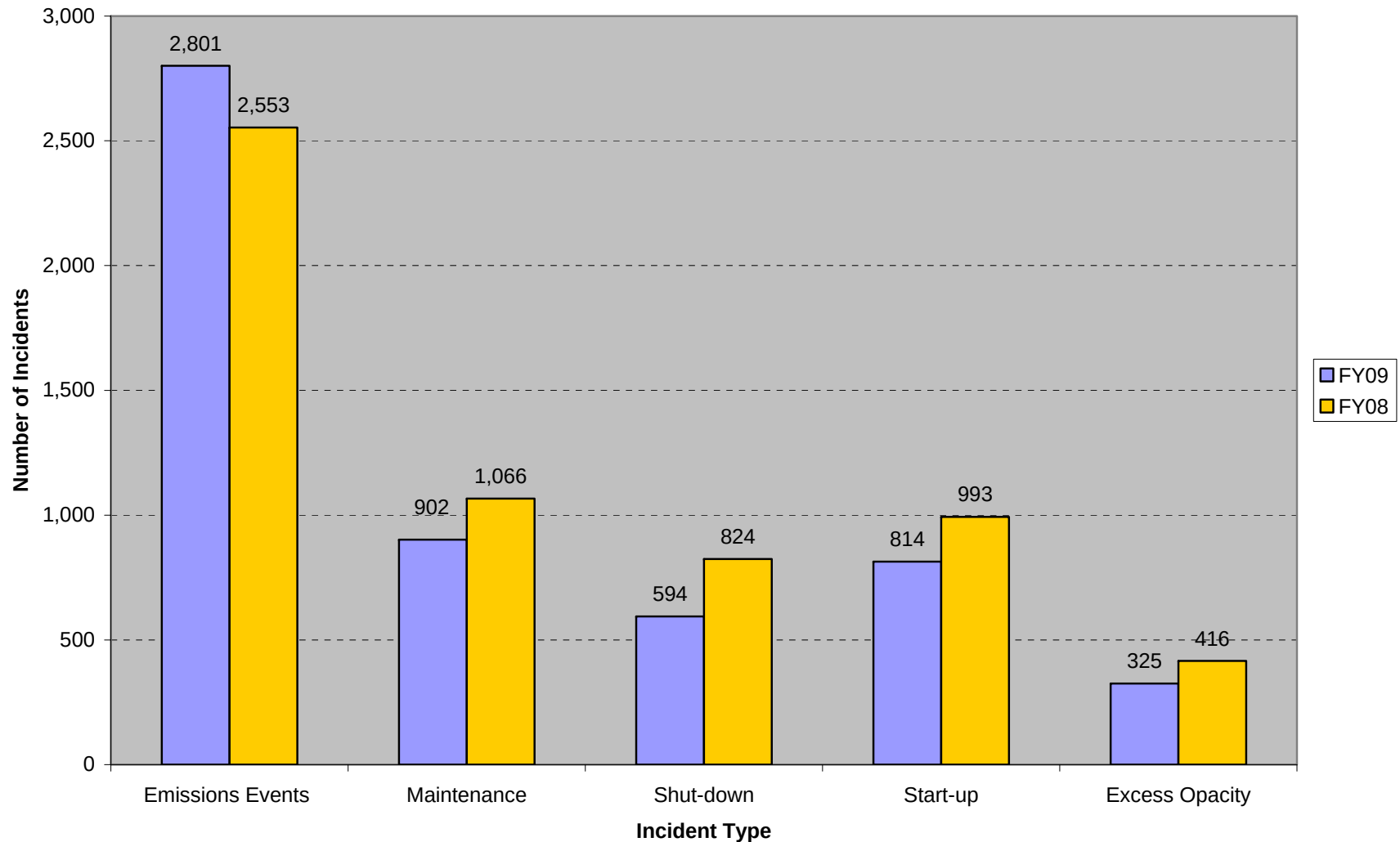
Figure 5-1 Reported Incidents
