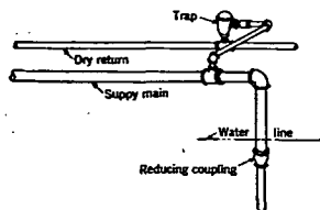
FIG. 33. DIPPING END OF MAIN INTO WET RETURN
