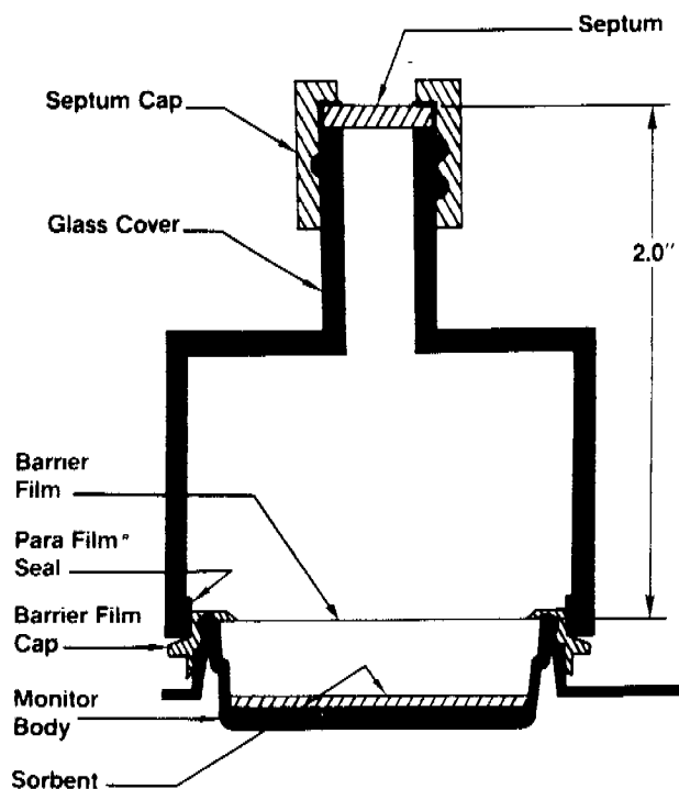
Figure 2 — Cylindrical glass dome for gas spiking
