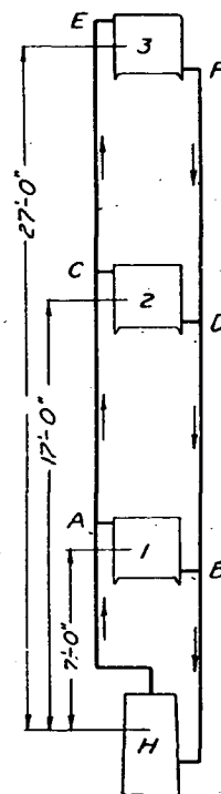
FIG. 35. GENERAL ARRANGEMENTS OF HEATING SYSTEM
