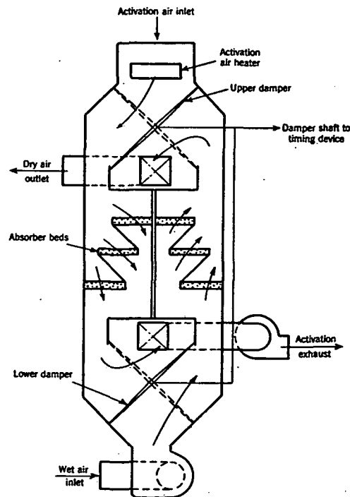
FIG. 5. SOLID ADSORBENT DEHYDRATOR—STATIONARY BED TYPE
