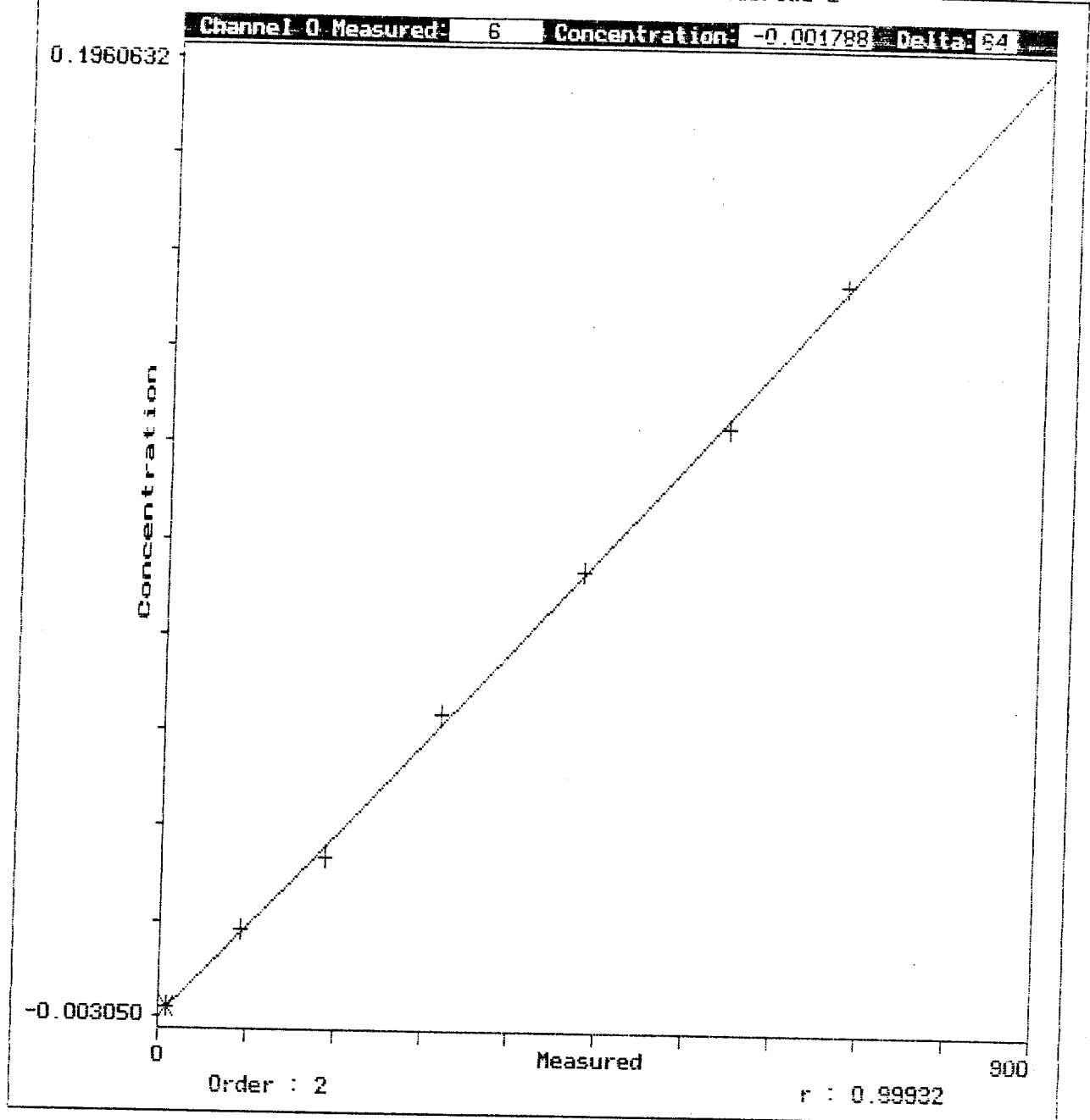
Calibration curve of 950502B1 : Fluoride L
