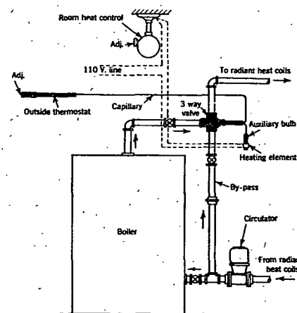
FIG. 12. TYPICAL PANEL AND RADIANT HEAT CONTROL SYSTEM
