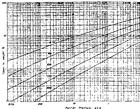
FIGURE 6 - ADSORPTION OF VINYL CHLORIDE ON BPL
