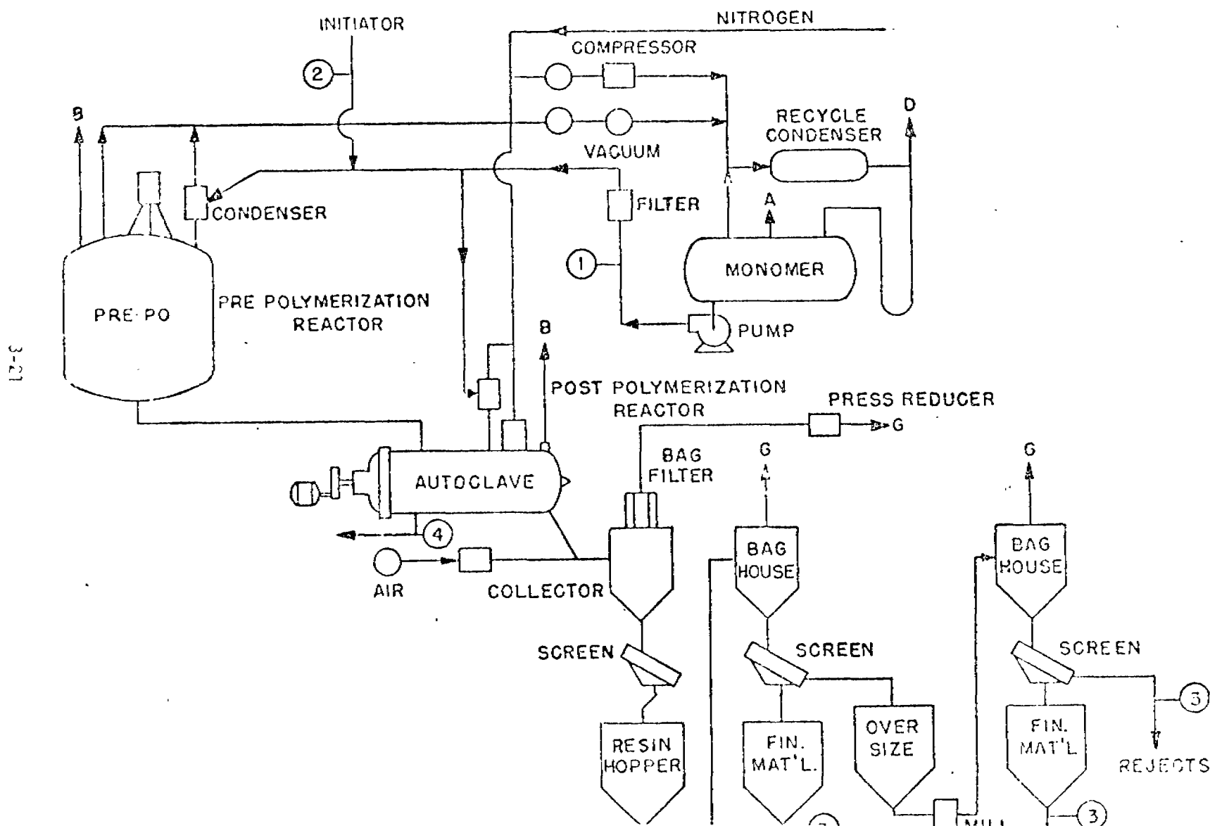
FLOW SHEET FOR POLYVINYL CHLORIDE BULK PROCESS 4/
