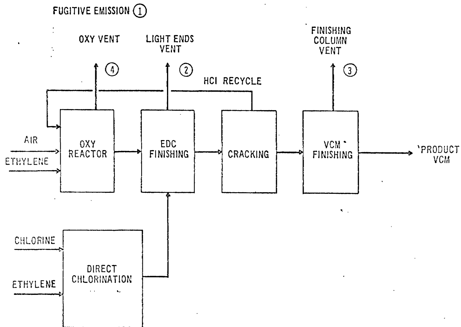
VINYL CHLORIDE BY THE BALANCED PROCESS
