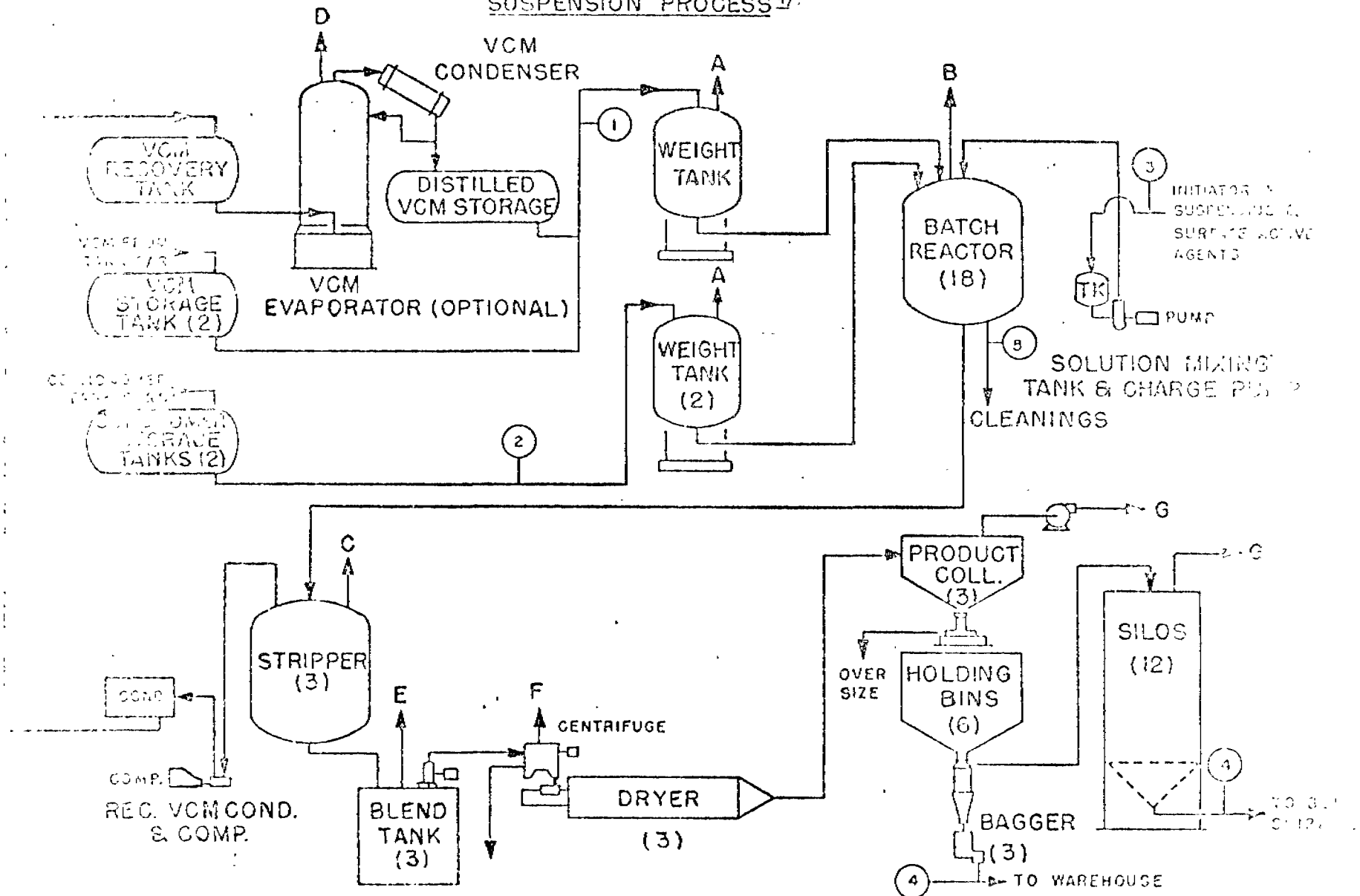
Figure 15 POLYVINYL CHLORIDE PLANT SUSPENSION PROCESS 4/
