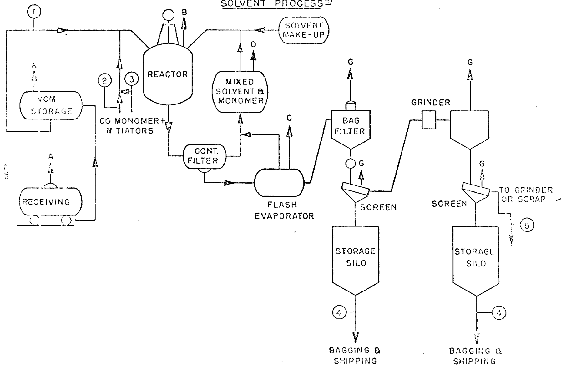
Figure 3-8 POLYVINYL CHLORIDE SOLVENT PROCESS 4/
