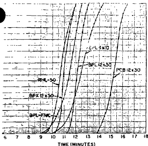
FIGURE 1 - 33% VINYL CHLORIDE IN AIR
