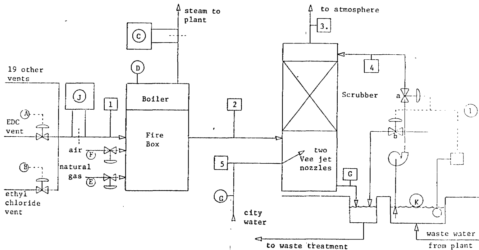
Figure 4-2. AMERICAN CHEMICAL INCINERATOR TEST, OCTOBER 7-9, 1974. (Data points--A,B,etc.; sample points--1,2,etc.)
