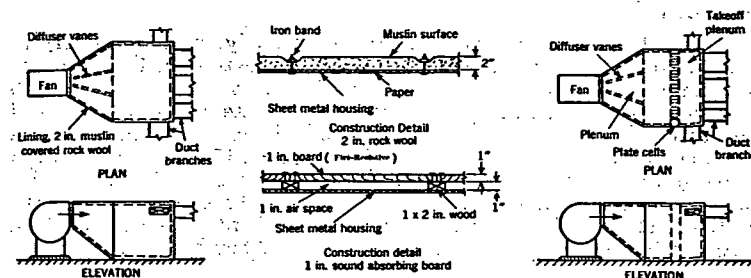
FIG. 1. ABSORPTION PLENUMS WITH AND WITHOUT SOUND CELLS
