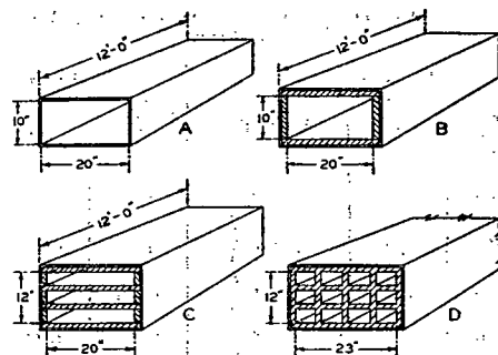
FIG. 6. ACOUSTIC TREATMENT OF DUCTS
