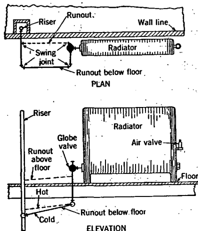
FIG. 7. TYPICAL ONE-PIPE RADIATOR CONNECTIONS (UP-FEED OR DOWN-FEED)
