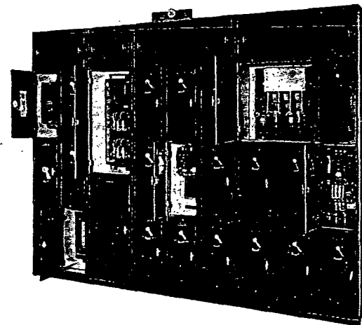
Typical Cabinetrol unit, showing open motor-starter panels
