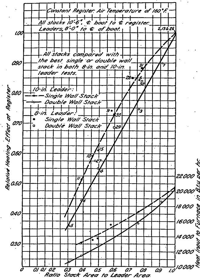
FIG. 50. RELATIVE HEATING EFFECT OF STACKS AT CONSTANT REGISTER AIR TEMPERATURE
