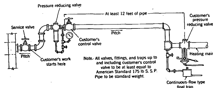
FIG. 4. STEAM SUPPLY CONNECTION WHEN USING TWO REDUCING VALVES
